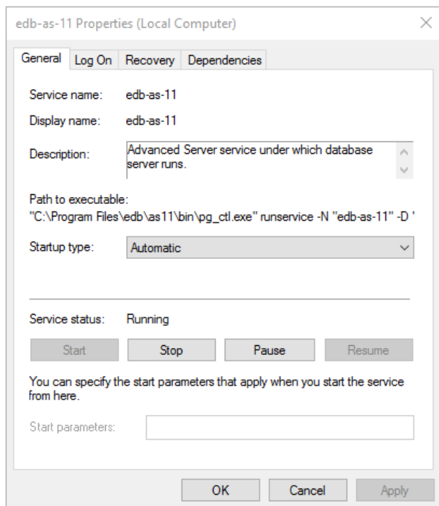
Fig. 2: Specifying Advanced Server's startup behavior
